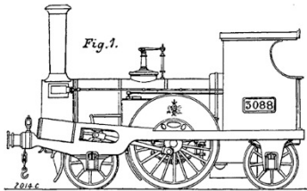
TREVITHICK'S PASSENGER ENGINE. BUILT 1848. COMPOUNDED BY F. W. WEBB 1879.
