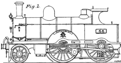
WEBB'S COMPOUND ENGINE. BUILT 1882.
