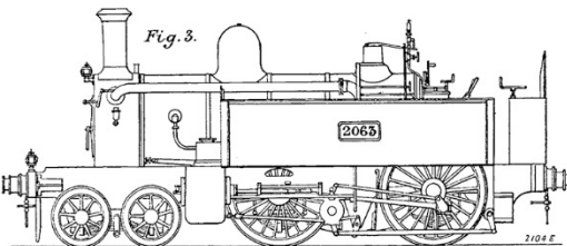
BEYER AND PEACOCK'S SIDE TANK ENGINE. COMPOUNDED BY F. W. WEBB, 1884.
