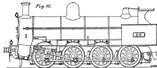
WEBB'S EIGHT-WHEELED COUPLED FREIGHT ENGINE. BUILT 1893.
