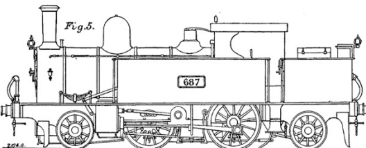
WEBB'S COMPOUND SIDE TANK PASSENGER ENGINE. BUILT 1885.
