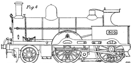
WEBB'S COMPOUND ENGINE. BUILT 1884.
