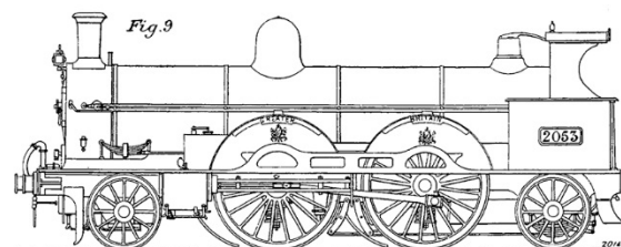
WEBB'S COMPOUND PASSENGER ENGINE, "GREATER BRITAIN." BUILT 1891.
