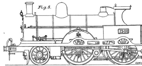
WEBB'S COMPOUND ENGINE, "TEUTONIC." BUILT 1889.
