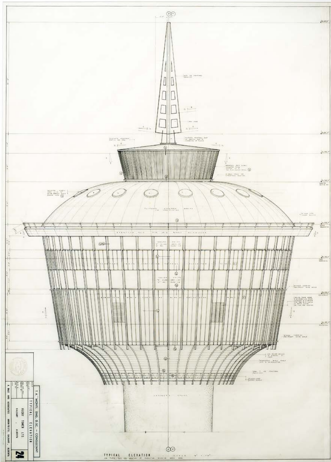
Chandler Kennedy, D. (1967). Typical Elevation of Calgary (Husky) Tower, Dale Chandler Kennedy fonds, 195A/84.16, Canadian Architectural Archives, Archives and Special Collections, University of Calgary.
