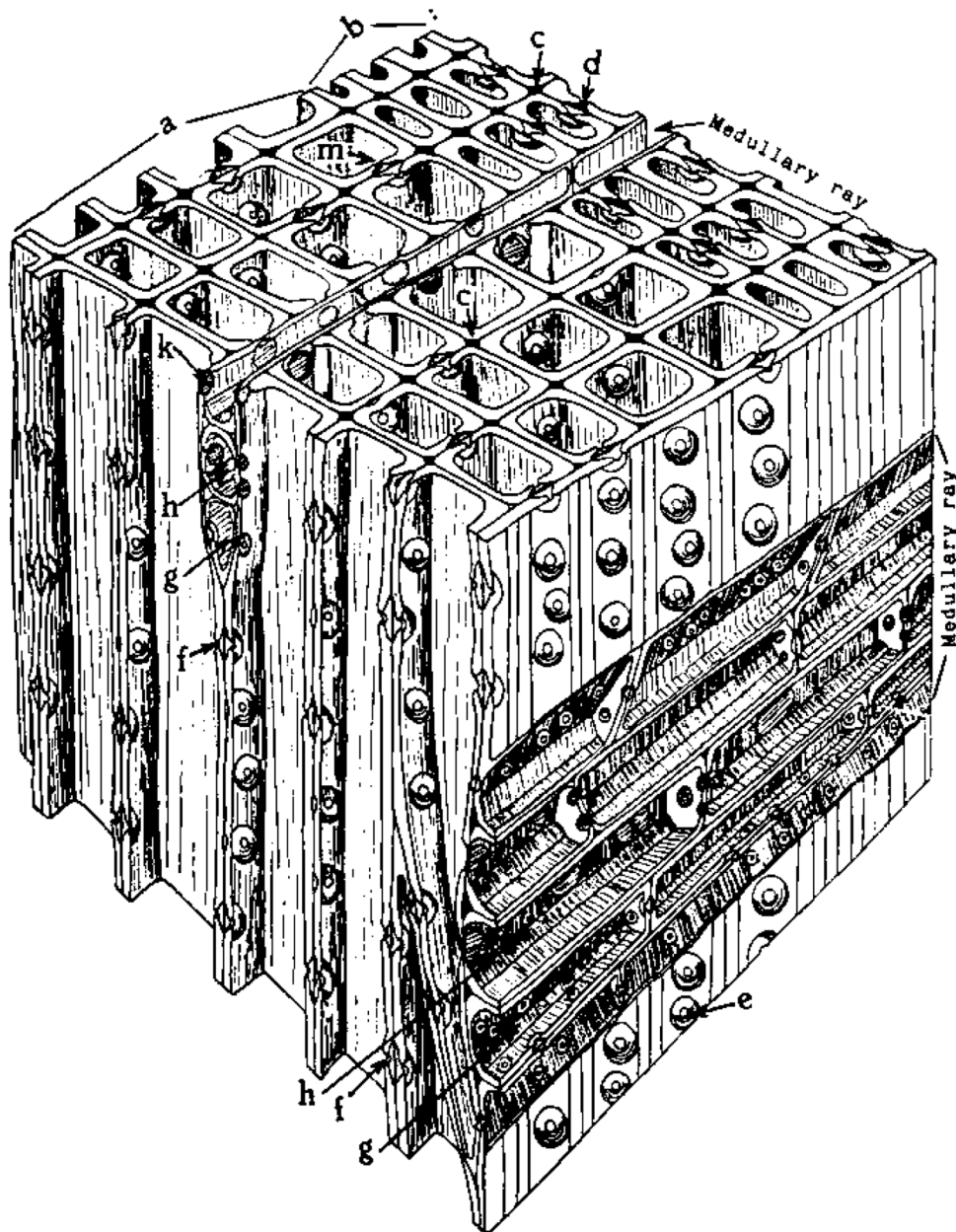
FIG. 55.—Diagrammatic representation of a block of pine wood highly magnified. a , Early growth; b , late growth; c , intercellular space; d , bordered pit in tangential wall of late growth; m , f and e , bordered pit in radial wall of early growth from different points of view; h , row of medullary cells for carrying food; g , row of medullary ray cells for carrying water; k , thin place in radial wall of ray cells that carry food.
