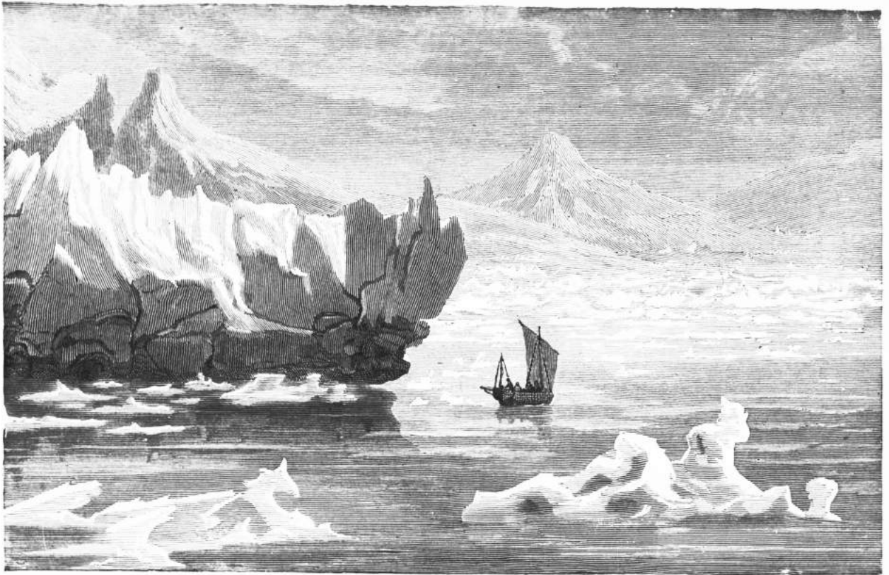
240. Glaciers in the Bay of the Magdalen, Spitzbergen.
