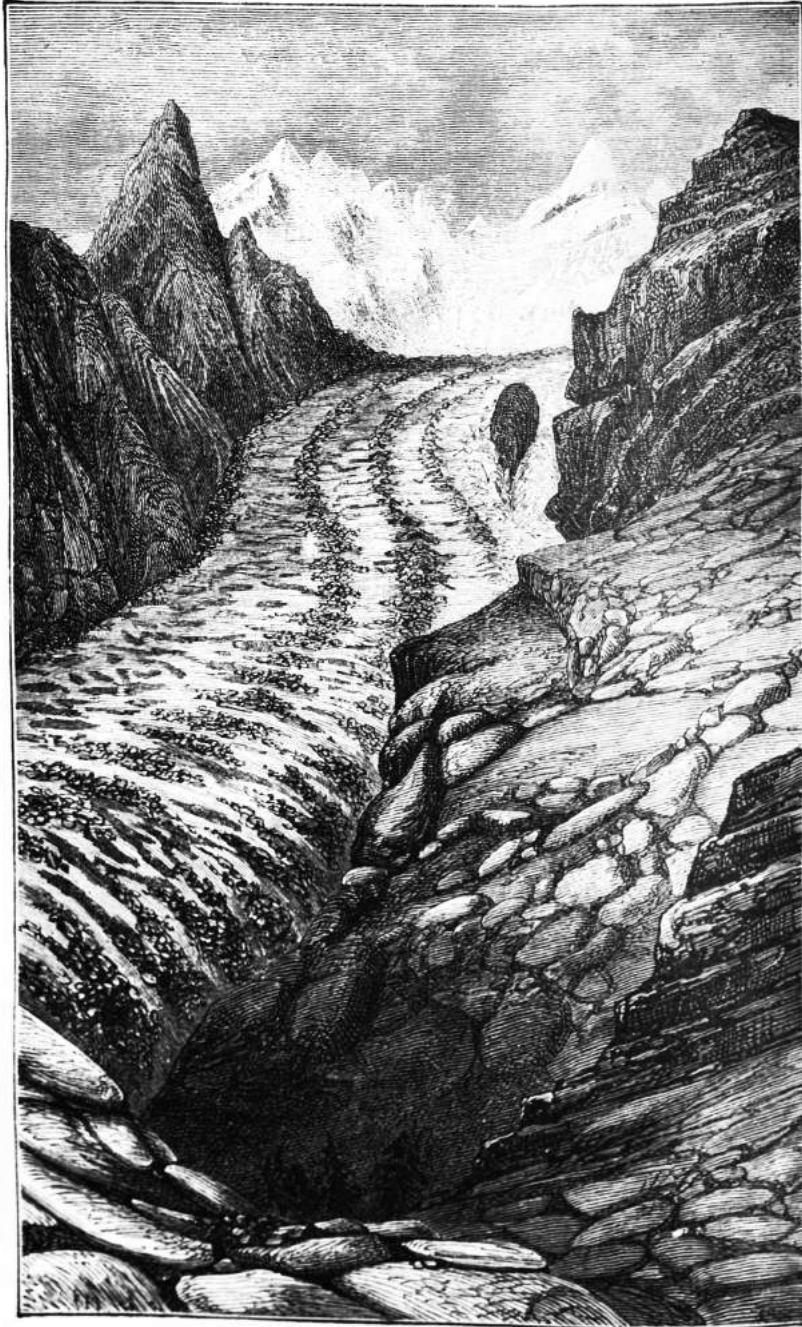
FIG. 39 - Glacier of Zermatt
